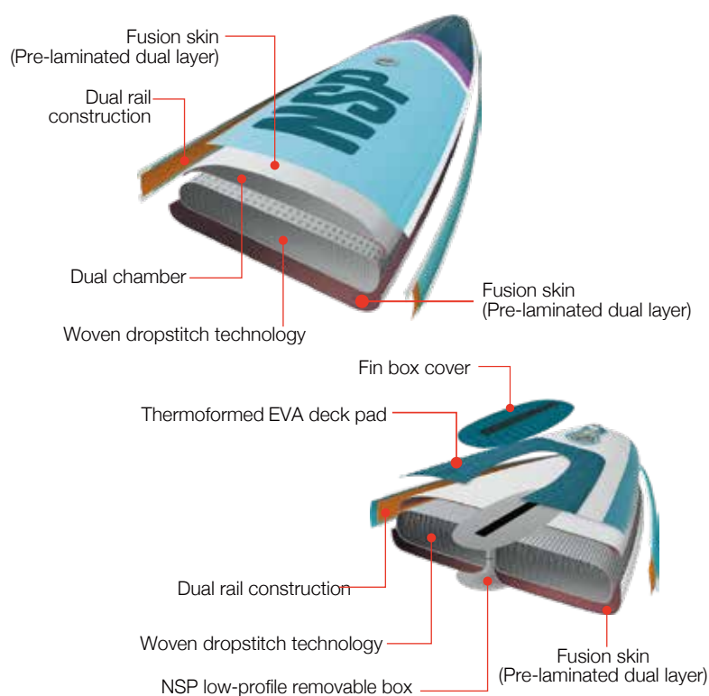
Low-profile Air7 V3 finbox system
