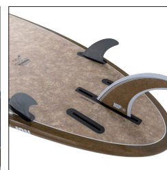
4 x FTU + 1 x US 10 finboxes
